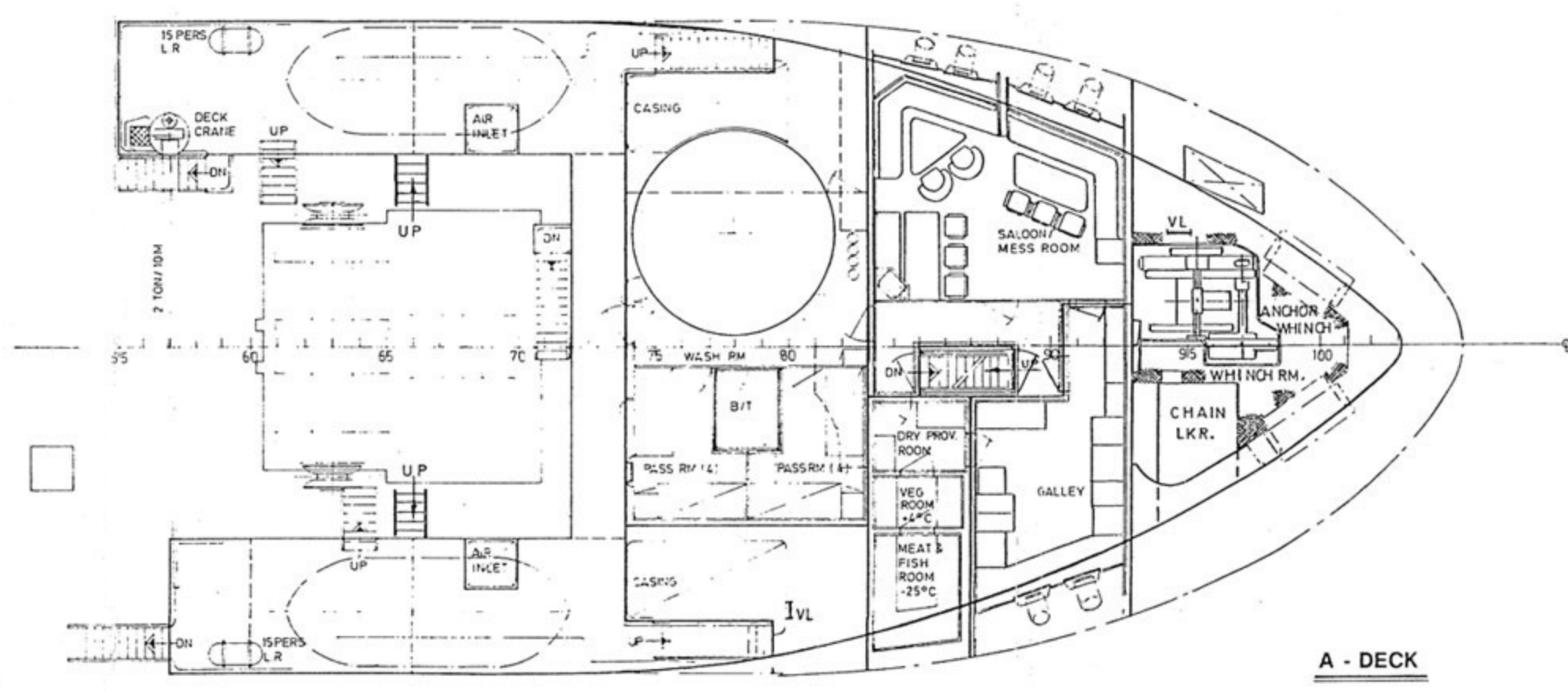
A - DECK
