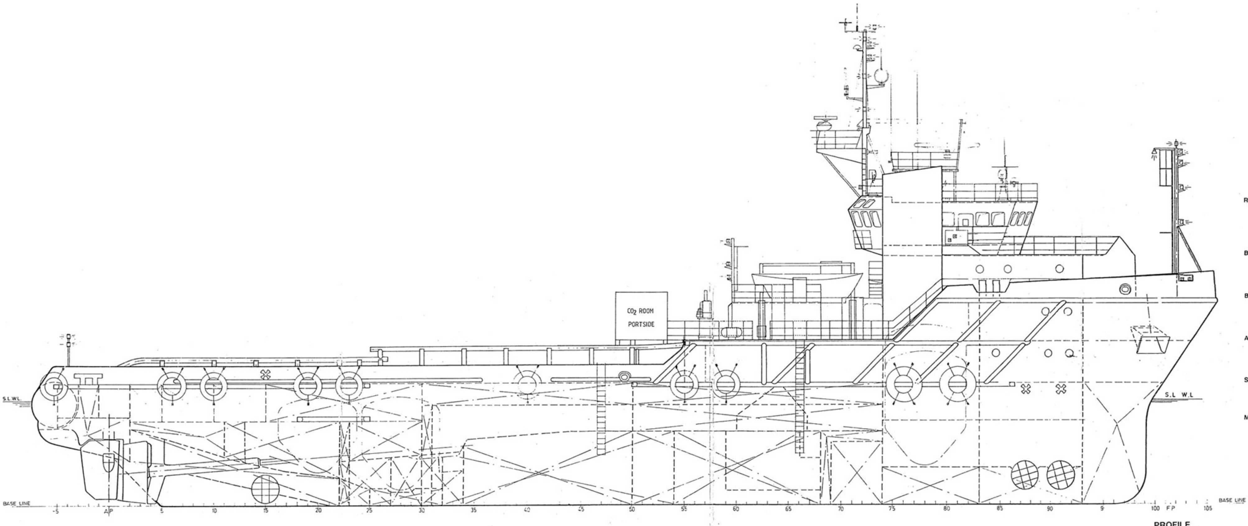
PROFILE
