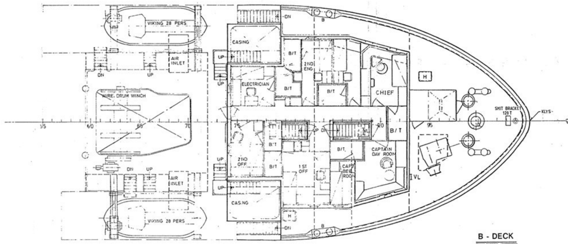
B - DECK
