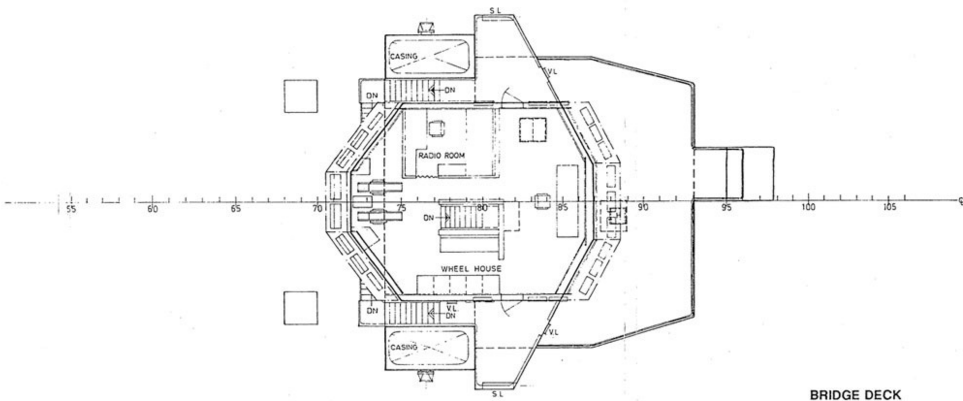
BRIDGE DECK
