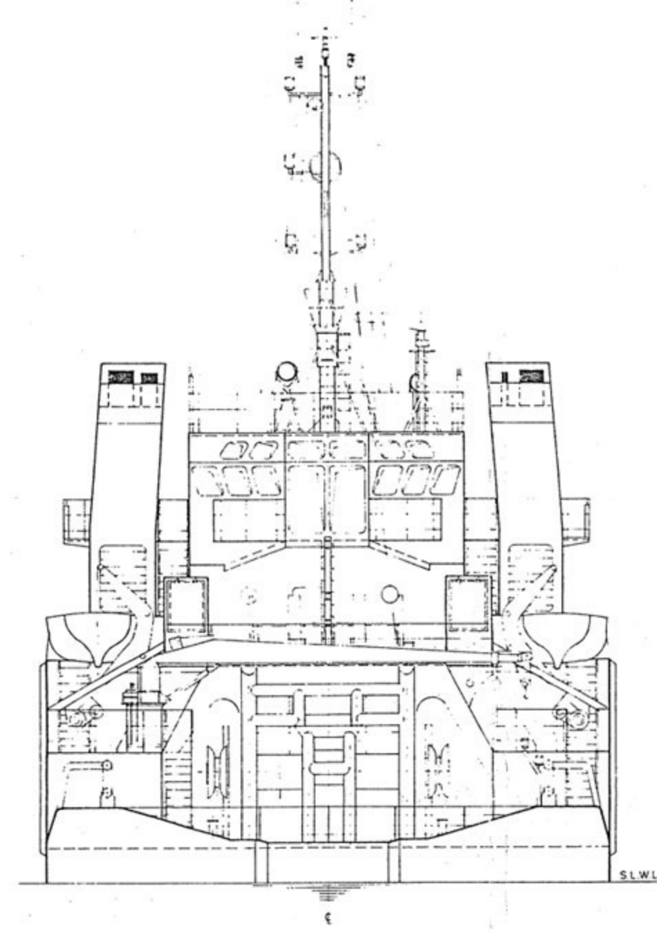
AFT VIEW
