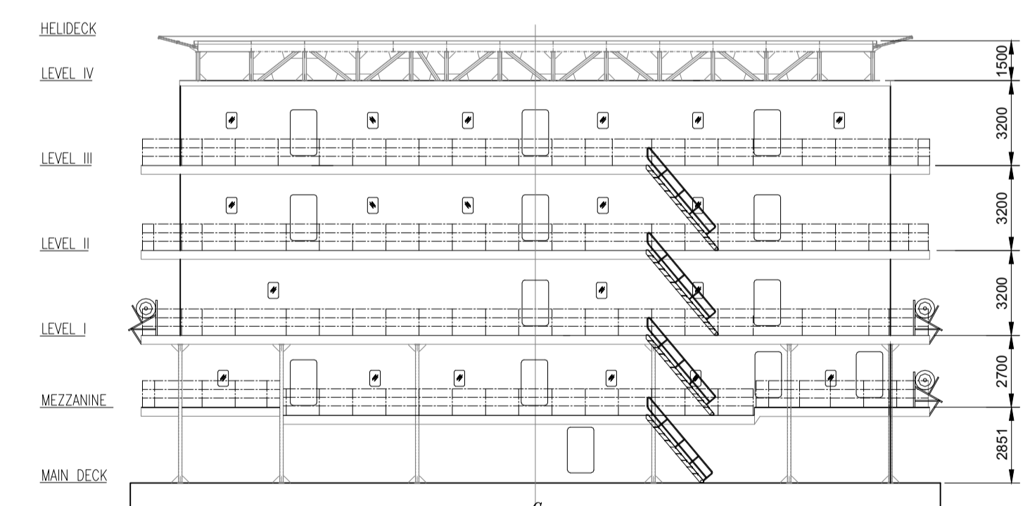
VIEW AT FR. 60 VIEW LOOKING AFT
