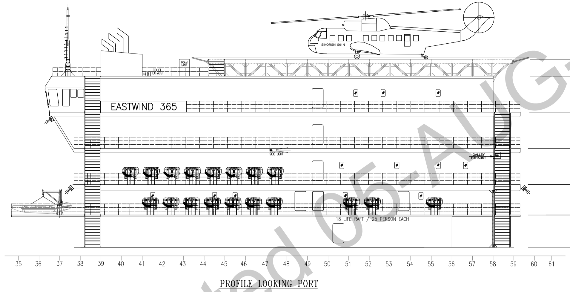
PROFILE LOOKING PORT
