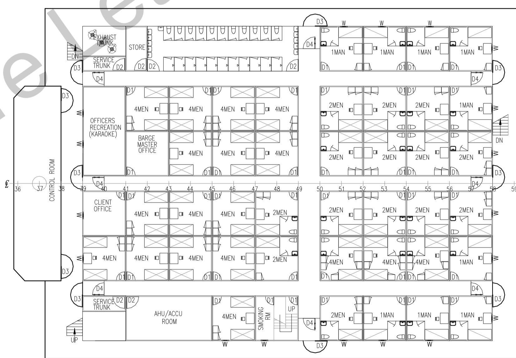
LEVEL III 1MAN x 09 = 09 2MEN x 14 = 28 4MEN x 18 = 72 CABIN TOILETS 23 No's COMMON TOILETS 11 No's
