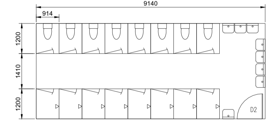
TYPICAL DET. OF COMMON TOILET
