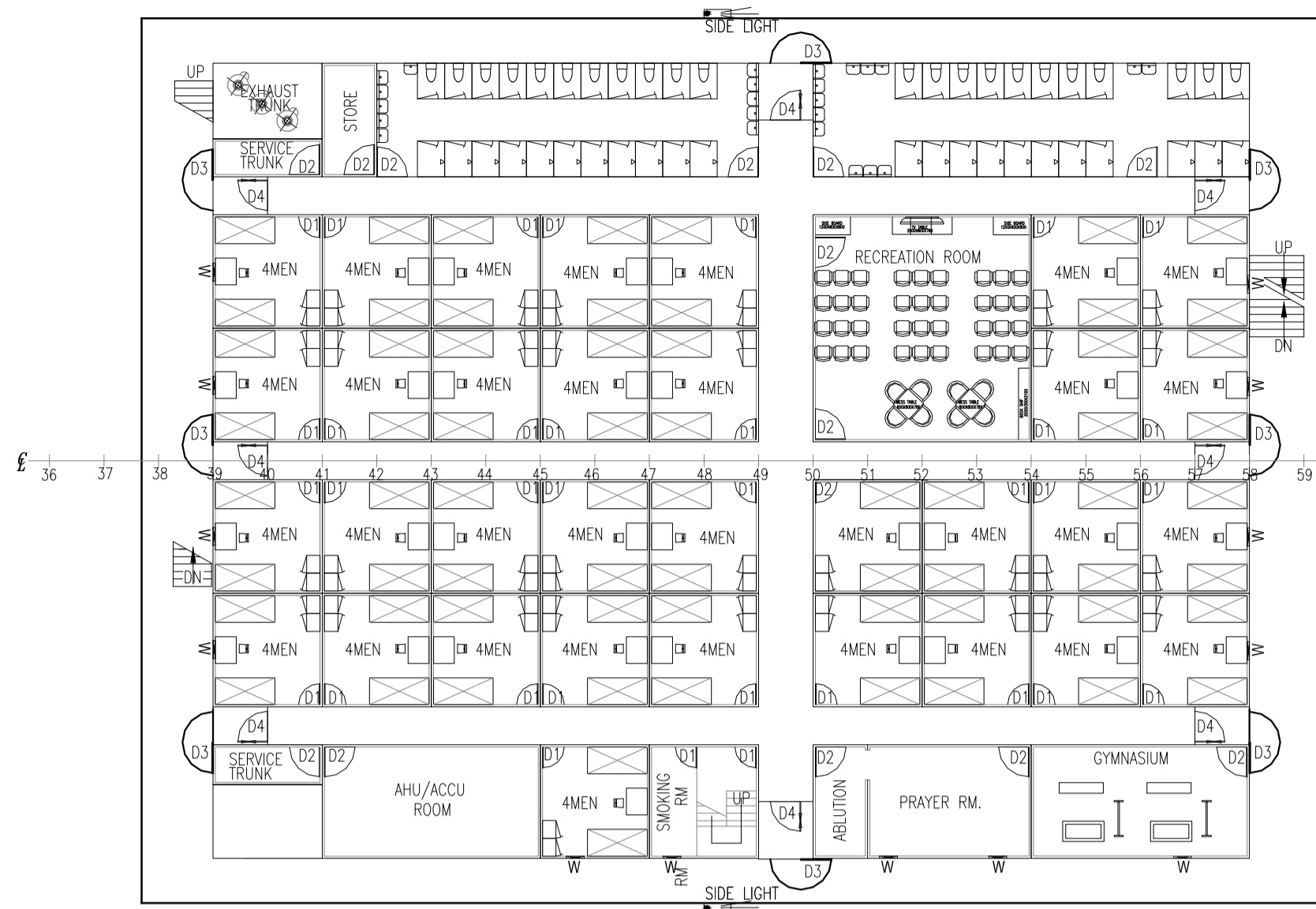
LEVEL II 4MEN x 33 = 132 COMMON TOILETS 22 No's
