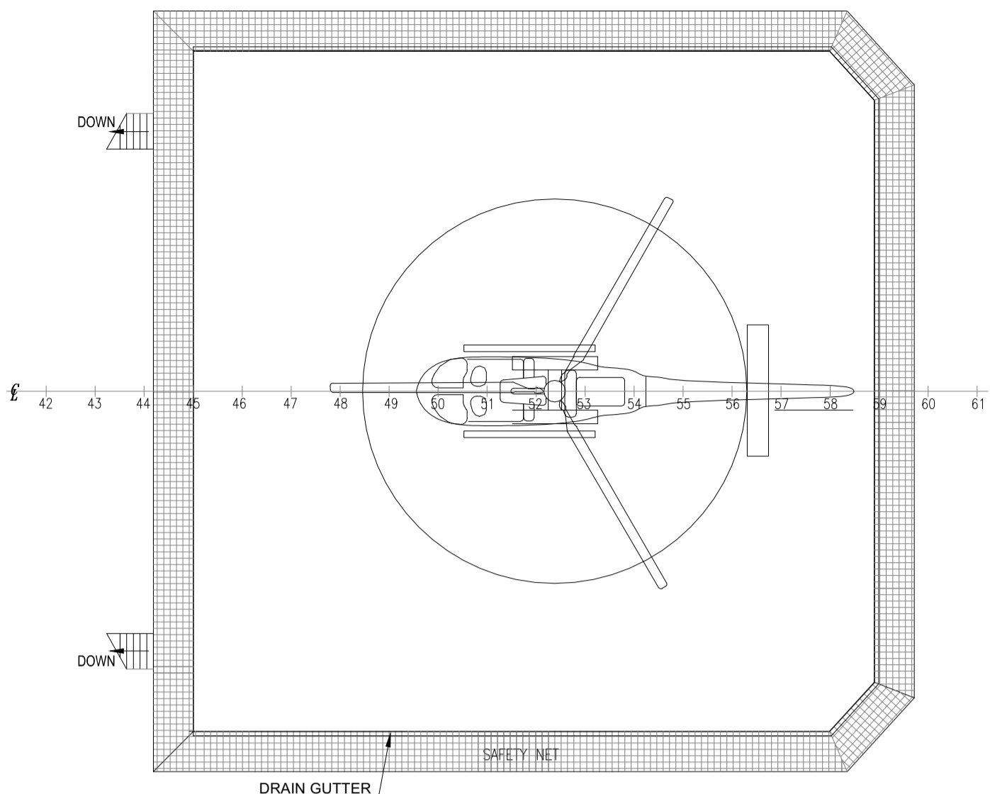
HELIDECK
