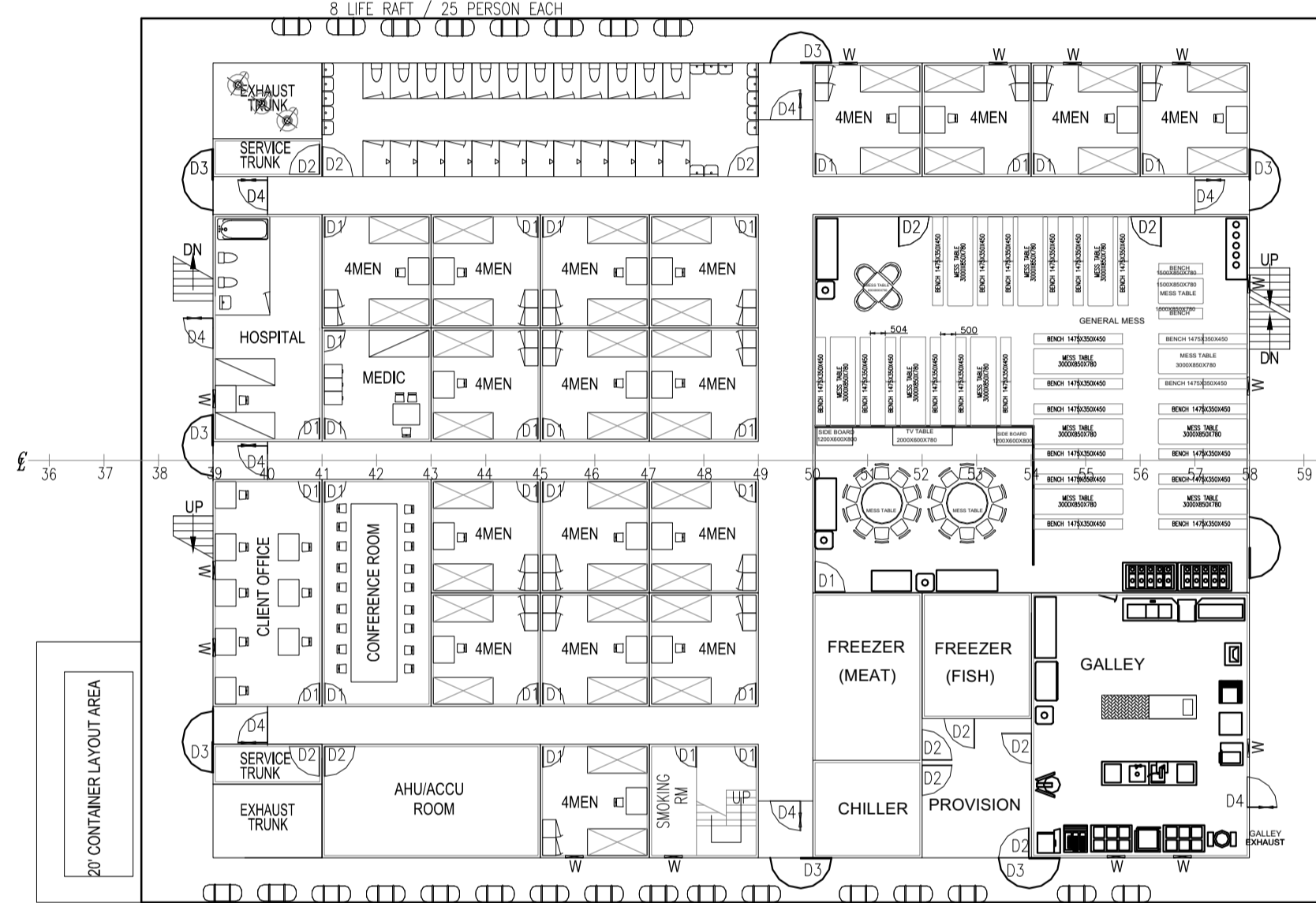
LEVEL I 4MEN x 18 = 72 COMMON TOILETS 12 No's
