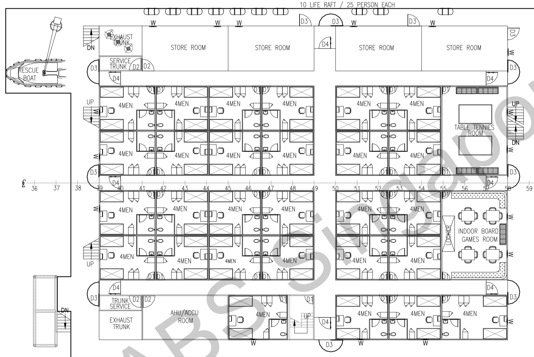
MEZZANINE LEVEL 4MEN x 28 = 112
