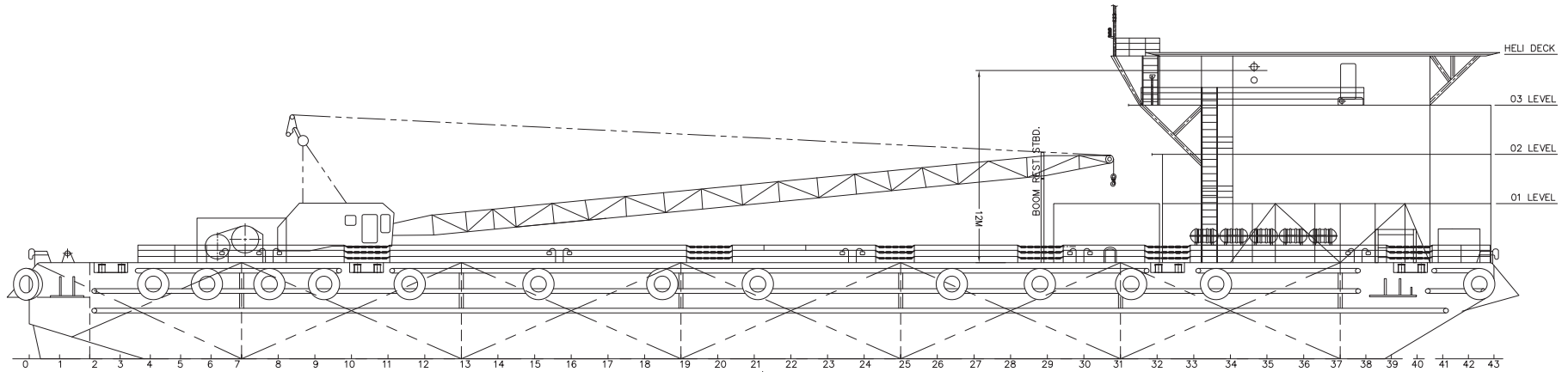
PROFILE
