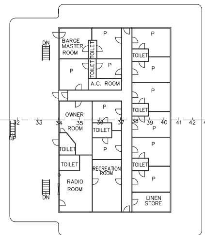
03 LEVEL DECK
