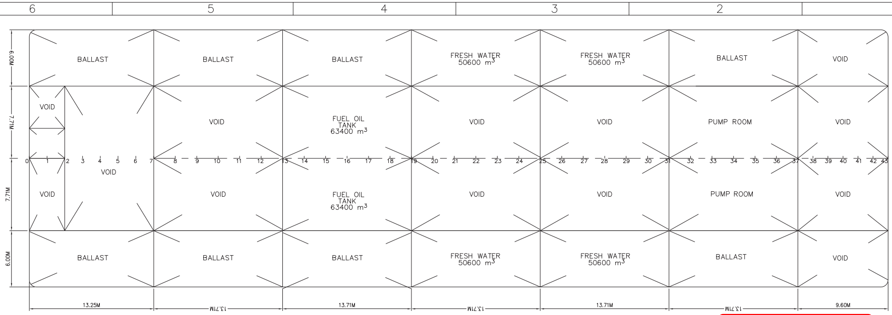
TANK PLAN
