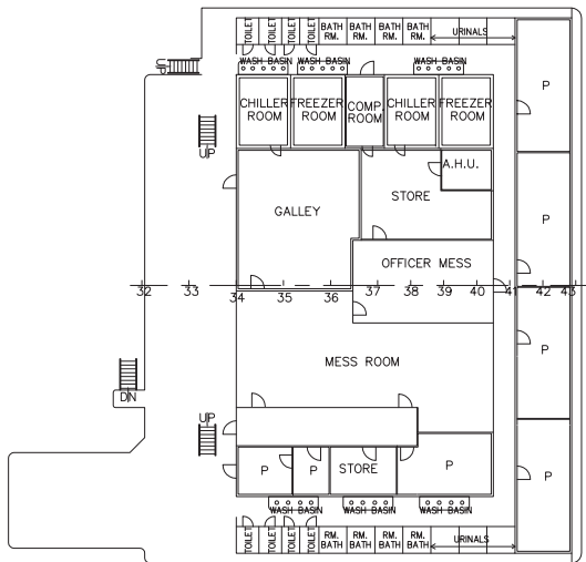
01 LEVEL DECK
