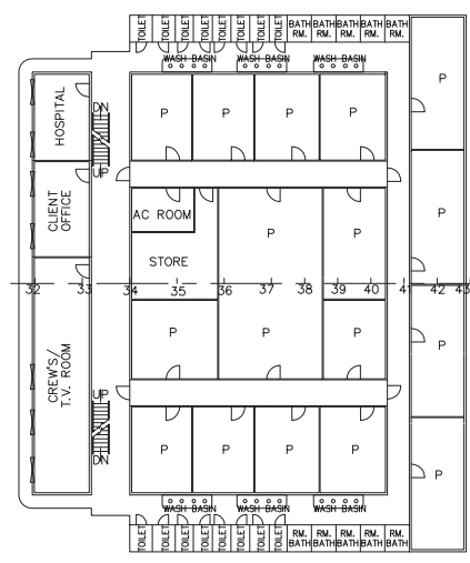
02 LEVEL DECK
