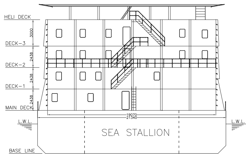
VIEW LOOKING FWD
