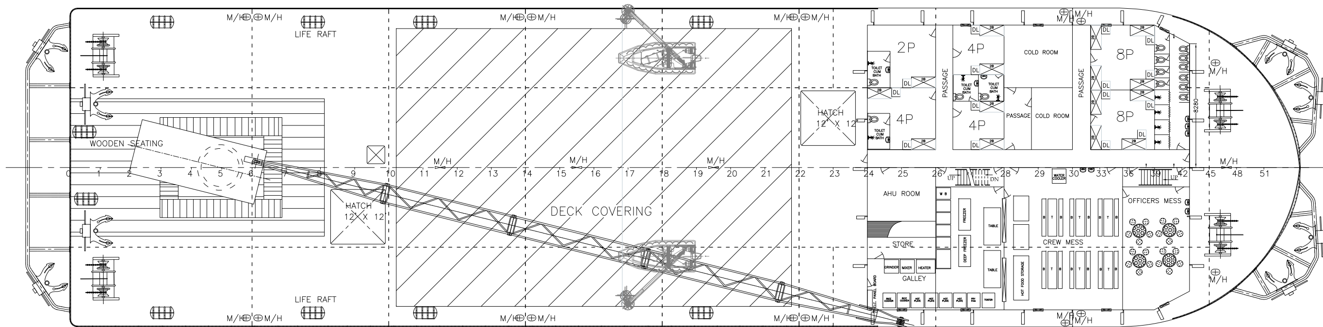
MAIN DECK 30 PERSON
