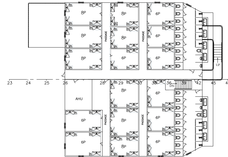
DECK - 3 (118 PERSONS)
