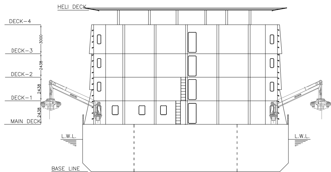
VIEW LOOKING AFT.
