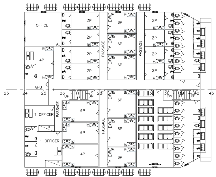
DECK - 1 (74 PERSONS)
