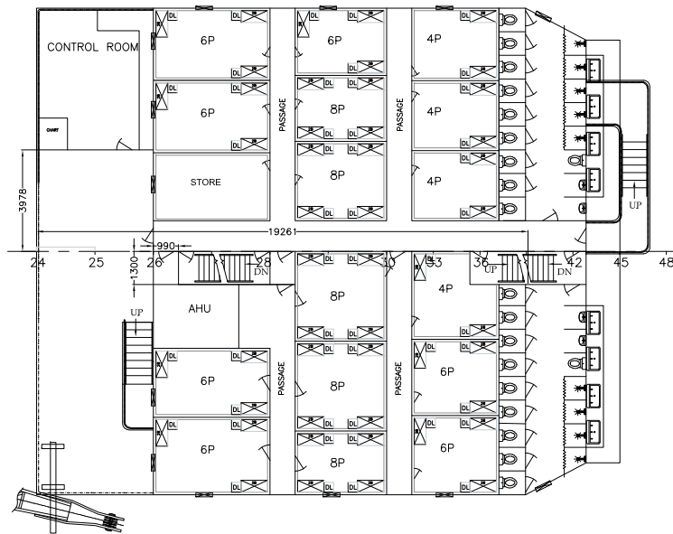
DECK - 2 (98 PERSONS)
