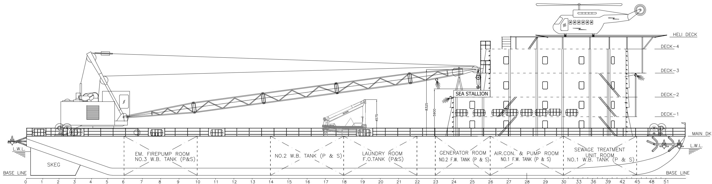
OUTBOARD PROFILE
